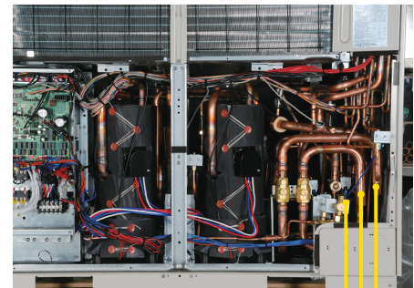
Liquid pipe Suction gas pipe Discharge gas pipe
